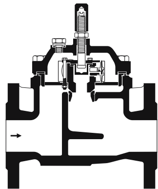
TK 23/24 DN 50
