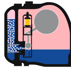
Air-venting when system is cold (start-up condition).
