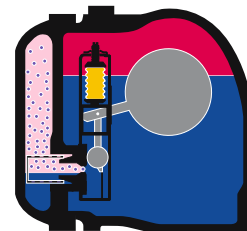
Discharge of boiling hot condensate (temperature equals saturation temperature).
