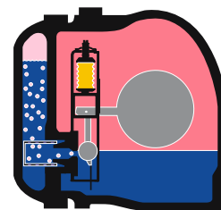
Air-venting during operation (temperature lower than standard steam temperature).
