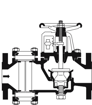
GK 11, 21
